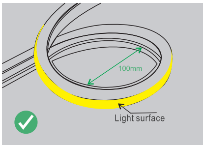
Light surface upwards, the strip is bendable to right or left naturally, the minimum bending diameter is 100mm.
